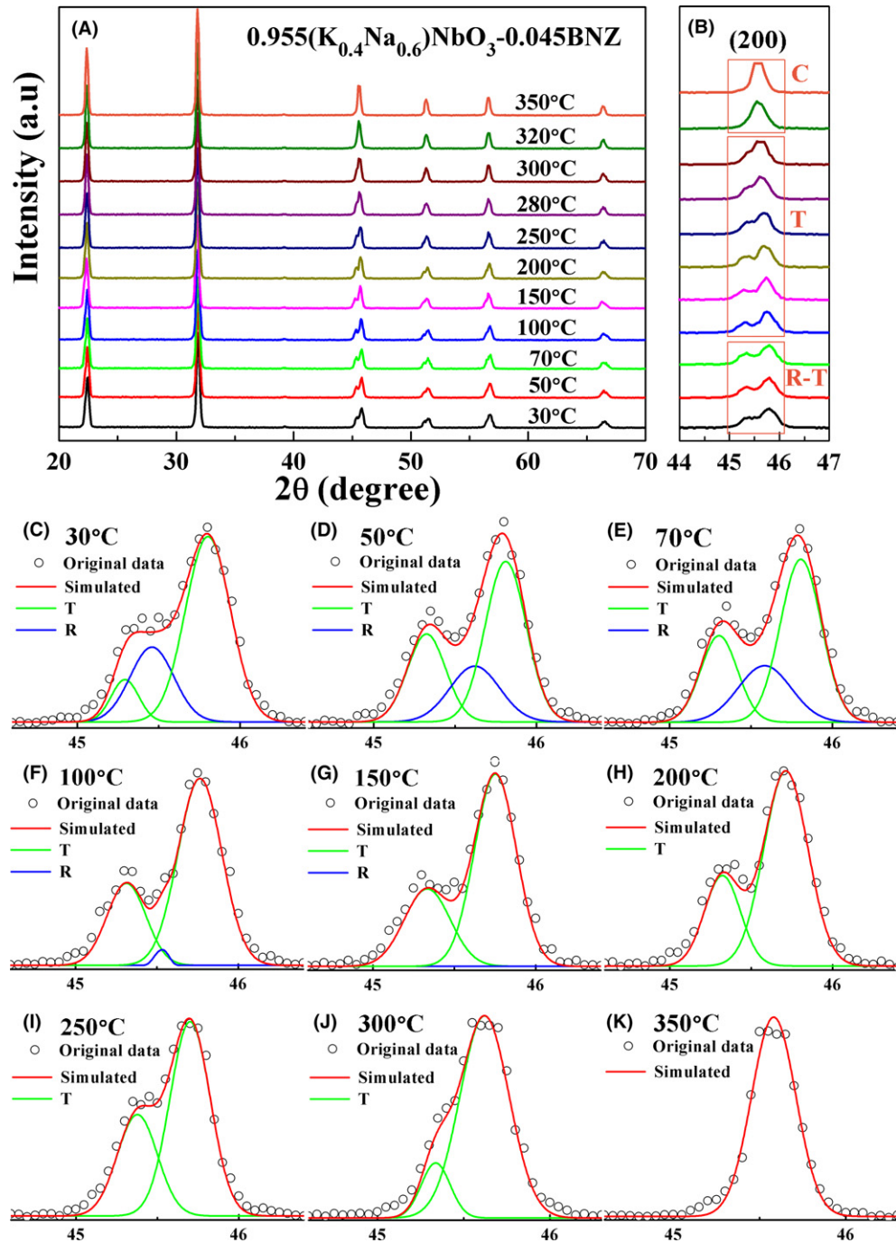
FIGURE 9 In situ temperature dependence of XRD patterns for KN0.6N-0.045BNZ (A) 2\theta=20^\circ-70^\circ , (B) 2\theta=44^\circ-47^\circ ; simulations of splitting of the {200} peaks with different temperatures (C) 30°C, (D) 50°C, (E) 70°C, (F) 100°C, (G) 150°C, (H) 200°C, (I) 250°C, (J) 300°C, and (K) 350°C [Color figure can be viewed at wileyonlinelibrary.com ]
