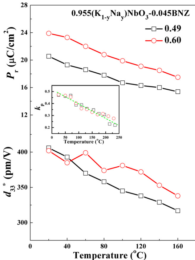
FIGURE 11 P_r and d_{33}^* as a function of temperature for KN0.49N-0.045BNZ and KN0.6N-0.045BNZ, inset shows the temperature dependence of k_p [Color figure can be viewed at wileyonlinelibrary.com]
