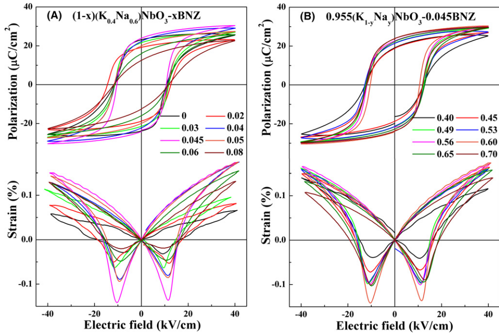
FIGURE 4 High electric field bipolar polarization hysteresis and strain loops for KNYN-xBNZ (A) KN0.6N-xBNZ and (B) KNYN-0.045BNZ [Color figure can be viewed at wileyonlinelibrary.com]
