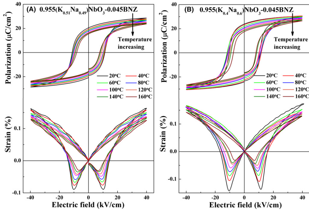
FIGURE 10 In situ temperature dependence of high electric field bipolar polarization hysteresis and strain loops for two MPB compositions (A) KN0.49N-0.045BNZ and (B) KN0.6N-0.045BNZ [Color figure can be viewed at wileyonlinelibrary.com]
