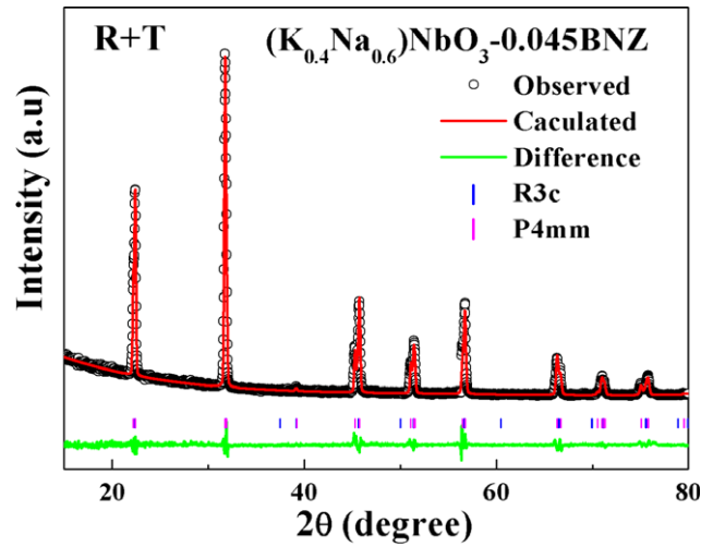
FIGURE 2 Rietveld refinement analysis of KN0.6N-0.045BNZ using the GSAS+EXPGUI package. Two phases R3c + P4mm were used. R_p=6.2\% , R_{wp}=9.7\% and \chi^2=1.88 [Color figure can be viewed at wileyonlinelibrary.com]
