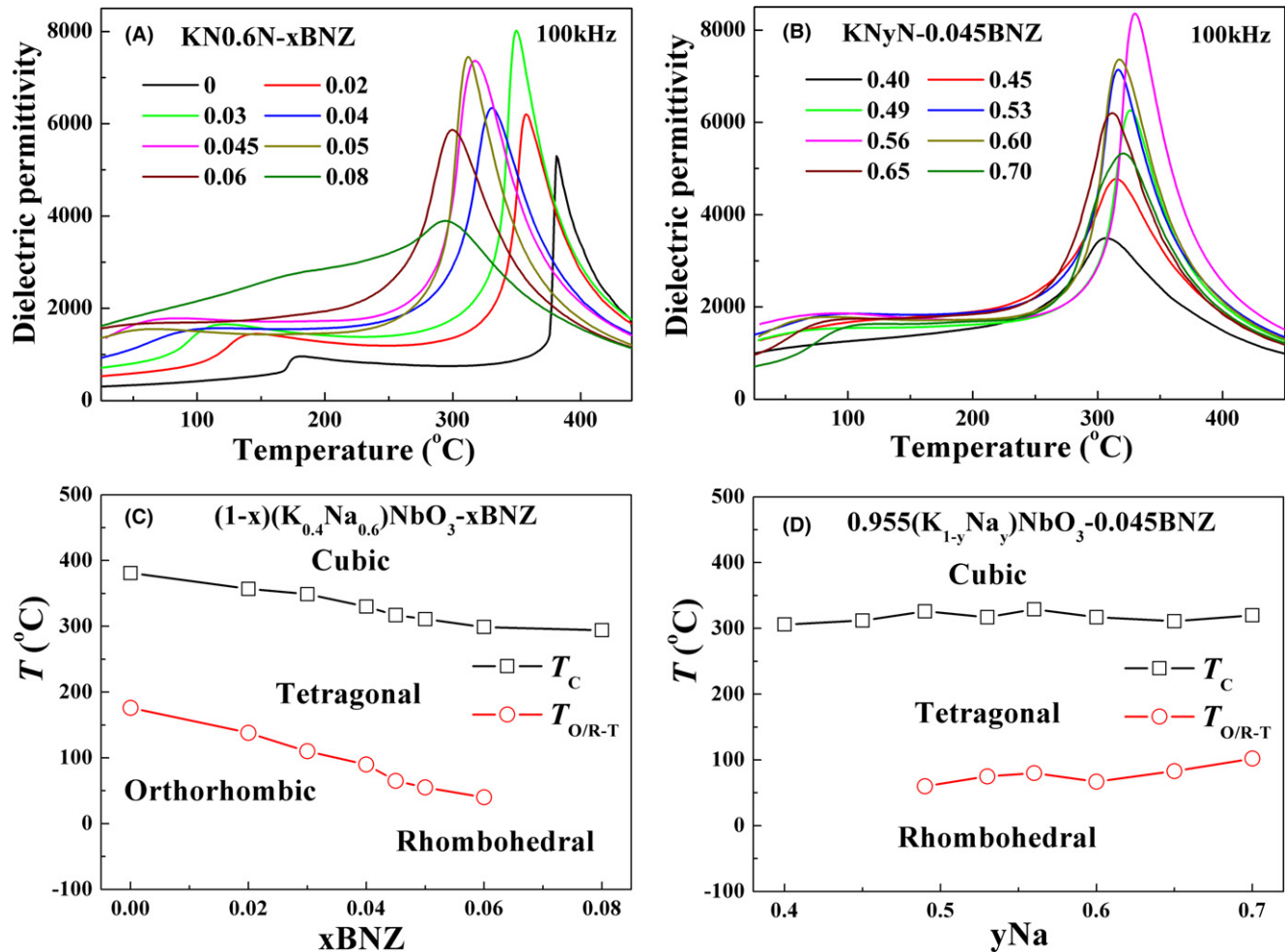
FIGURE 7 Temperature dependence of \epsilon_r and \tan\delta for \text{KNyN-xBNZ} (A) \text{KN}_{0.6}\text{N-xBNZ} , (B) \text{KNyN-0.045BNZ} , (C) T_C and T_{O/R-T} as a function of BNZ, (D) (C) T_C and T_{O/R-T} as a function of Na [Color figure can be viewed at wileyonlinelibrary.com ]
