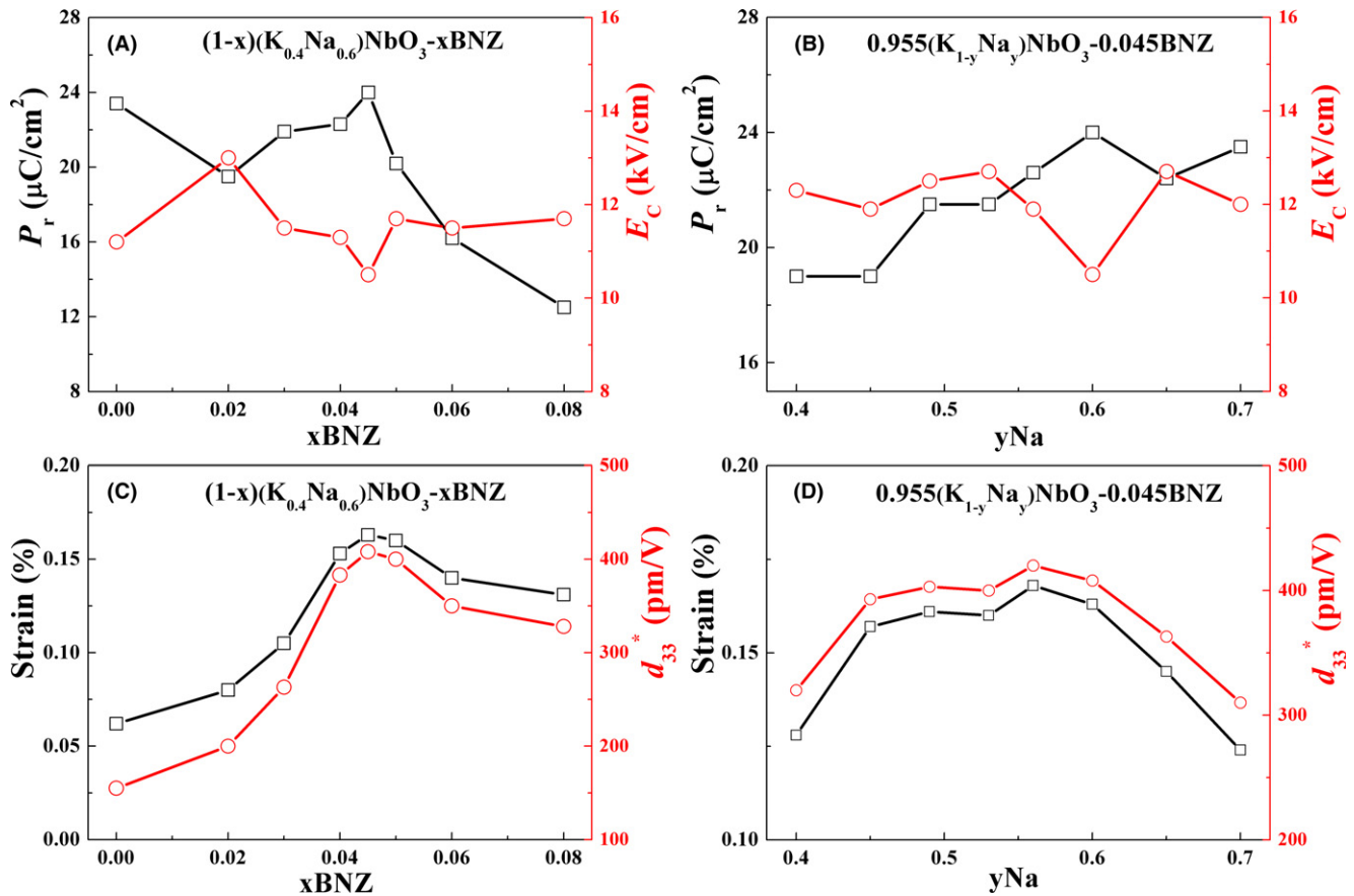
FIGURE 5 Ferroelectric and strain properties of KNYN-xBNZ (A) P_r and E_C as a function of BNZ, (B) P_r and E_C as a function of Na, (C) S and d_{33}^* as a function of BNZ, (D) S and d_{33}^* as a function of Na [Color figure can be viewed at wileyonlinelibrary.com]
