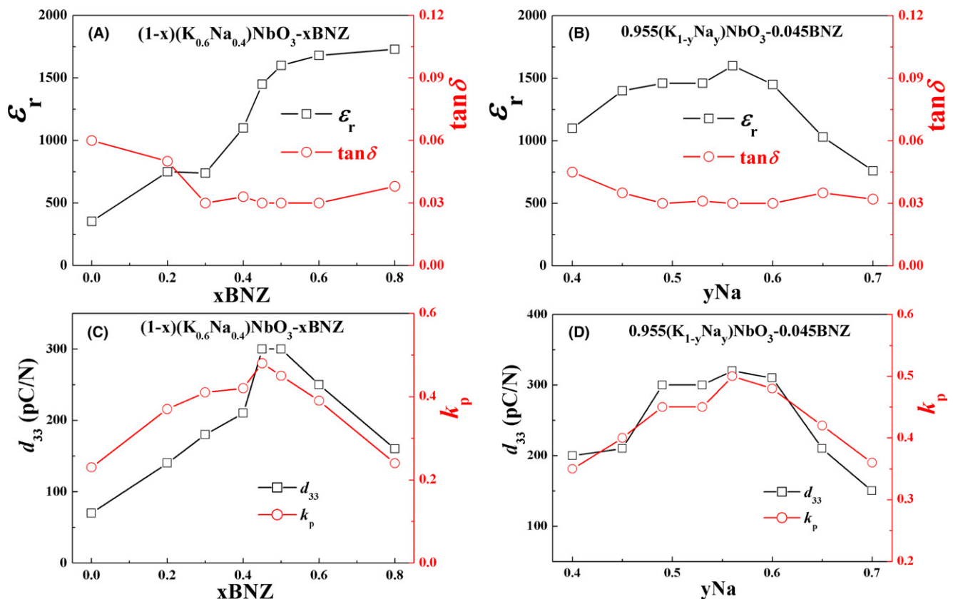
FIGURE 6 Dielectric and piezoelectric properties of \text{KNyN-xBNZ} (A) \epsilon_r and \tan\delta as a function of BNZ, (B) \epsilon_r and \tan\delta as a function of Na, (C) d_{33} and k_p as a function of BNZ, (D) d_{33} and k_p as a function of Na [Color figure can be viewed at wileyonlinelibrary.com ]
