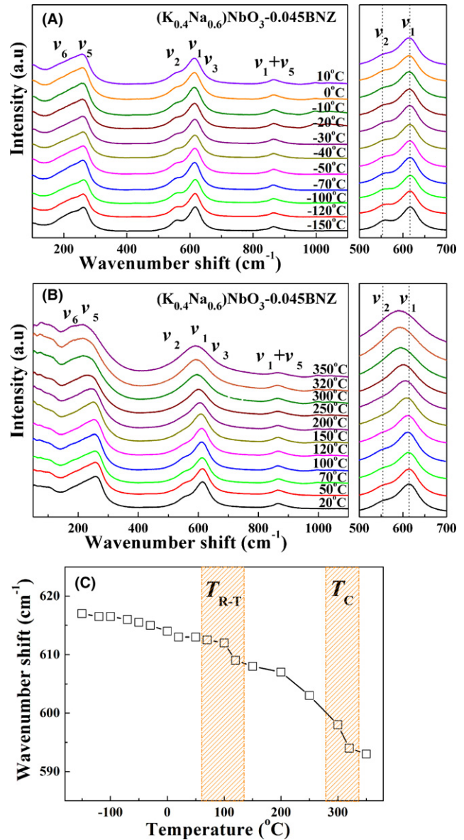
FIGURE 8 In situ temperature dependence of Raman spectra for \text{KN0.6N-0.045BNZ} (A) -150^\circ\text{C} - 10^\circ\text{C} , (B) 20^\circ\text{C} - 350^\circ\text{C} , (C) \nu_1 peak shift as a function of temperature [Color figure can be viewed at wileyonlinelibrary.com ]
