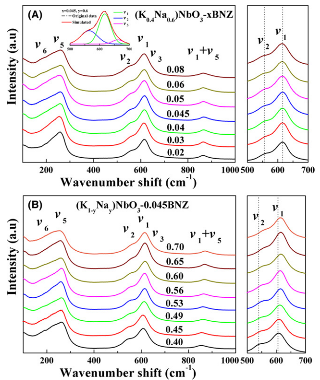
FIGURE 3 Room temperature Raman spectra of KNYN-xBNZ (A) KN0.6N-xBNZ, inset shows the Raman amplified peaks around 600 \text{cm}^{-1} simulated by Gaussian and (B) KNYN-0.045BNZ [Color figure can be viewed at wileyonlinelibrary.com]
